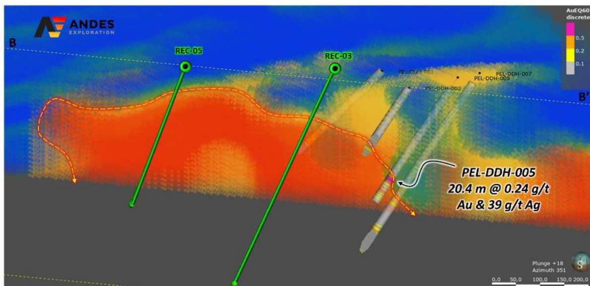
Figure 10: Marcelina High-Impact Depth Target Beneath Preserved Silica Cap, Defined by Coincident Geophysics and Drilling
