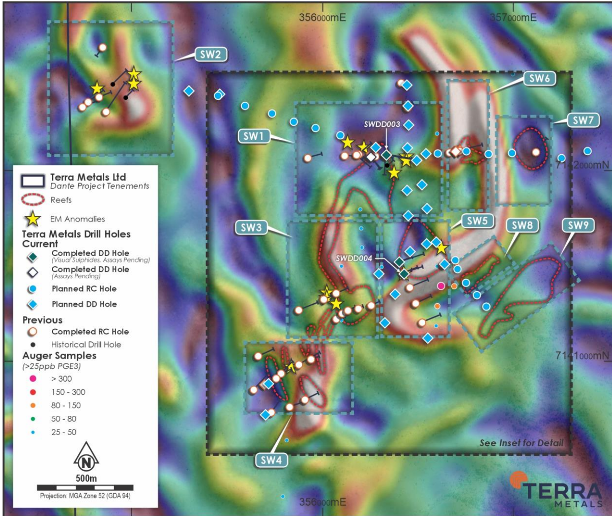
Figure 10. Plan view of the Southwest Prospect area, showing various target areas (SW1, SW2, SW3, SW4, SW5, SW6, SW7, SW8, SW9), over a mid-late time ground EM (historical) image.
