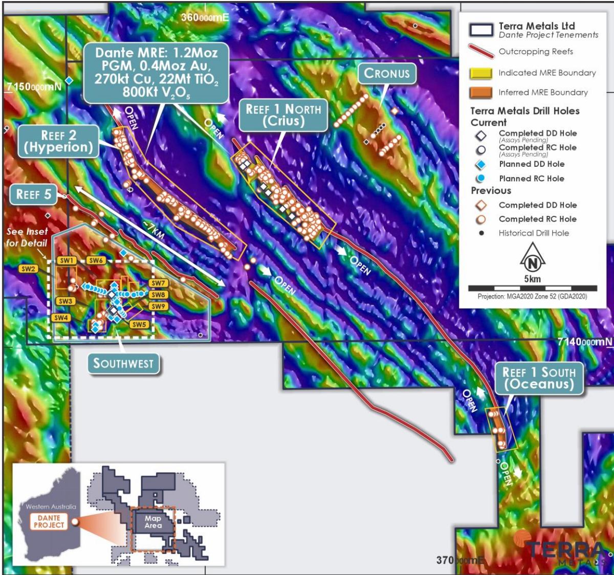
Figure 9. Plan view of Dante Project showing current MRE and the Southwest Prospect area.
