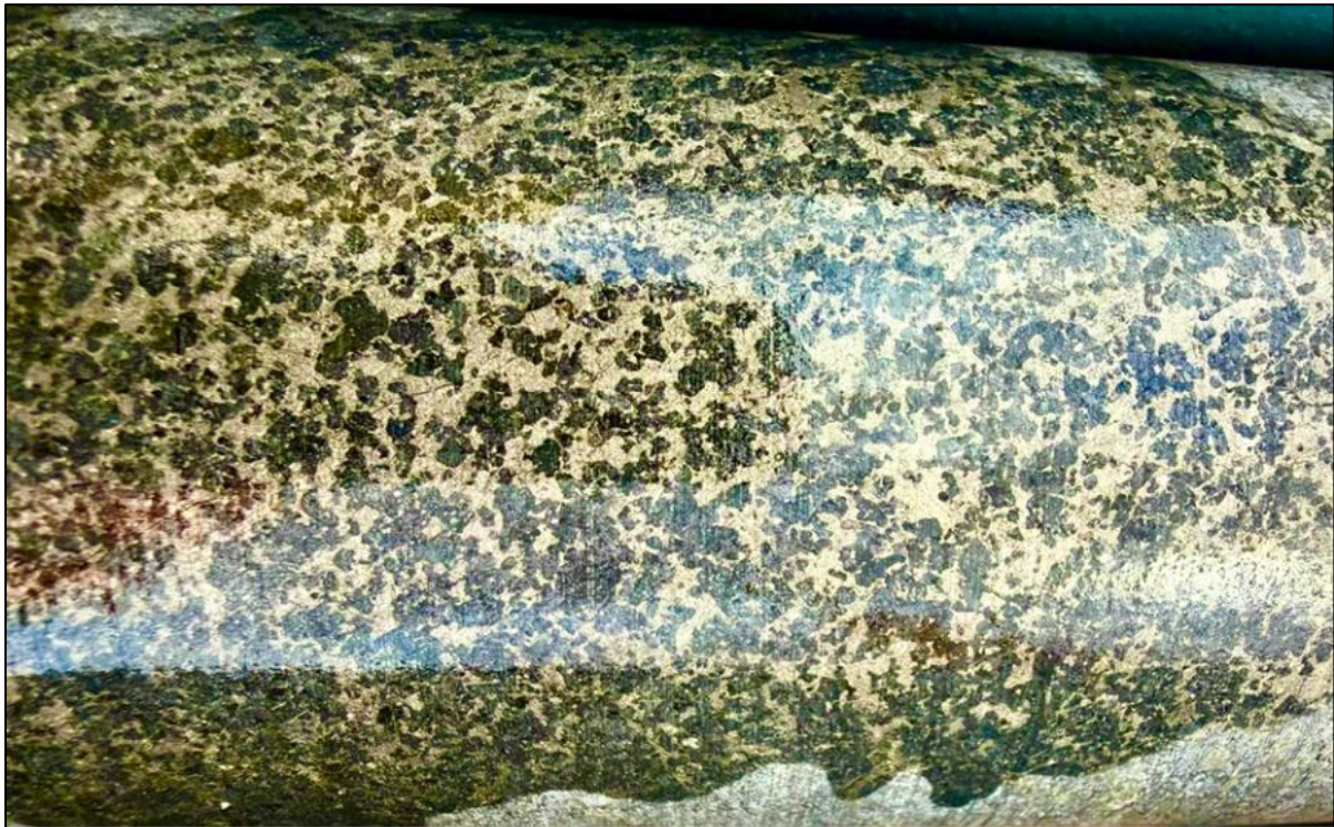
Figure 2. Semi-massive magmatic sulfide from SWD009 (from 66.5 m), PQ core diameter 85mm (8.5cm).
