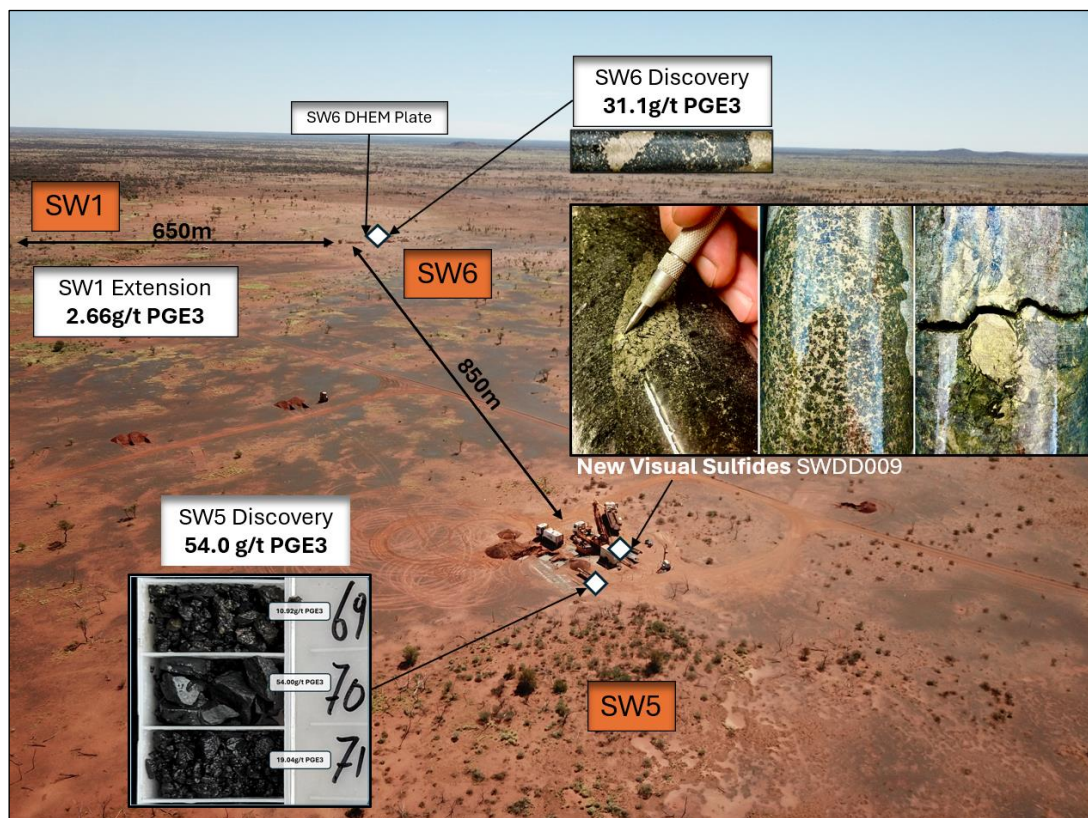
Figure 1. Aerial view of the SW5 and SW6/SW1 prospects at Southwest, showing the locations of the two discovery holes and the current diamond drill rig twinning discovery hole SWT008, which ended at 102m. Visual semi-massive sulfides have been intersected at depths between 60–80m, with drilling planned to 1,000m EOH depth.
