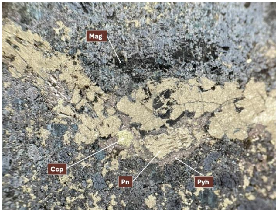
Figure 7. Magnified image of blebby and disseminated magmatic sulfide including pyrrhotite (Pyh), pentlandite (Pn), chalcopyrite (Ccp) and magnetite (Mag) within a gabbroic host rock. From SWD009 (from 52 m), field of view 50mm.
