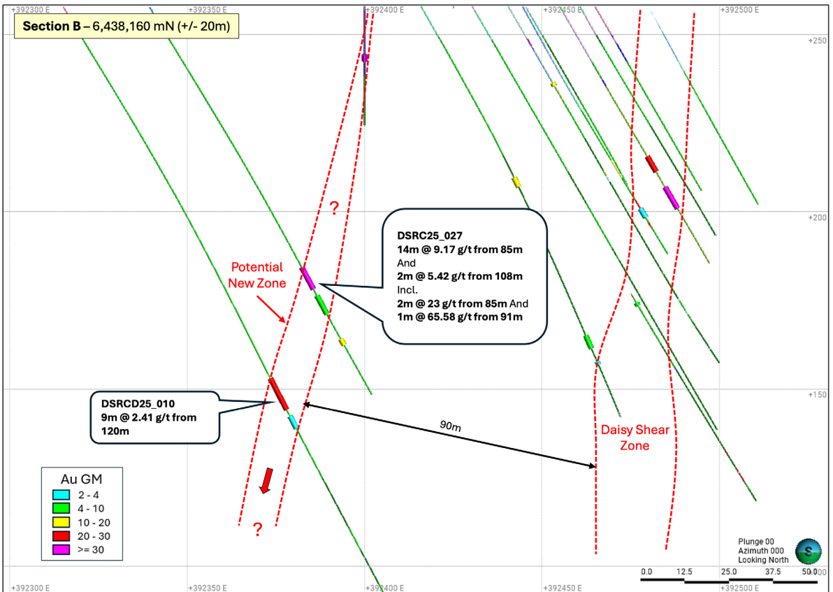
Figure: Daisy South extensions cross section B.
