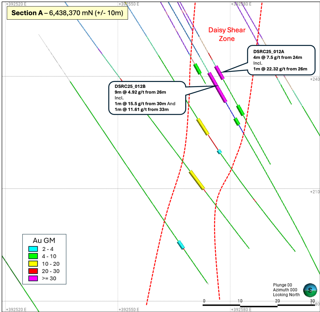
Figure: Daisy South extensions cross section A.
