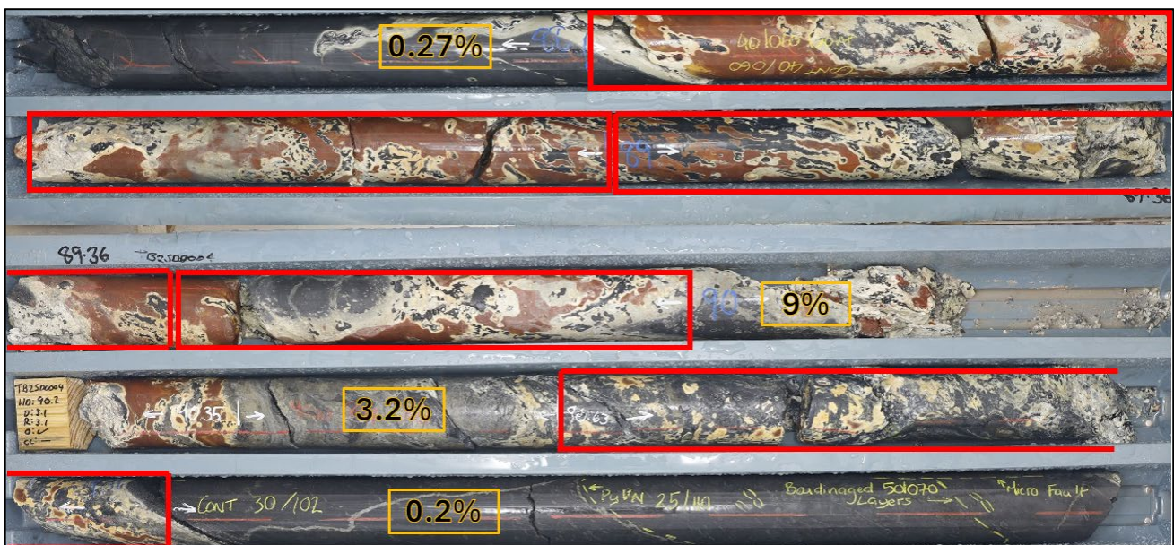
Figure 4 – Uraniferous mineralisation at 88m down hole in TB25DD004. Red boxes denote sample intervals that are pending. Assays received to date are shown in orange boxes. Assays pending are from 88-90m and 90.63-91m. Uraninite/pitchblende has partially to wholly replaced semi-massive pyrite and host volcaniclastic sediments forming clay (illite) and hematite. The mineralised interval is hosted within sericite altered tuffs and interbedded volcaniclastic arenites.
