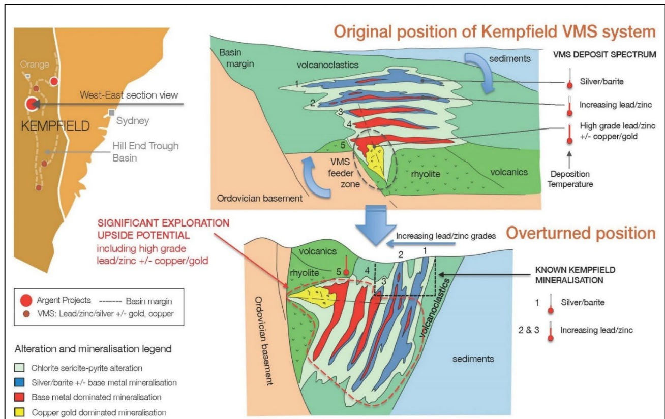
Figure 5 – Geological Model of Kempfield
