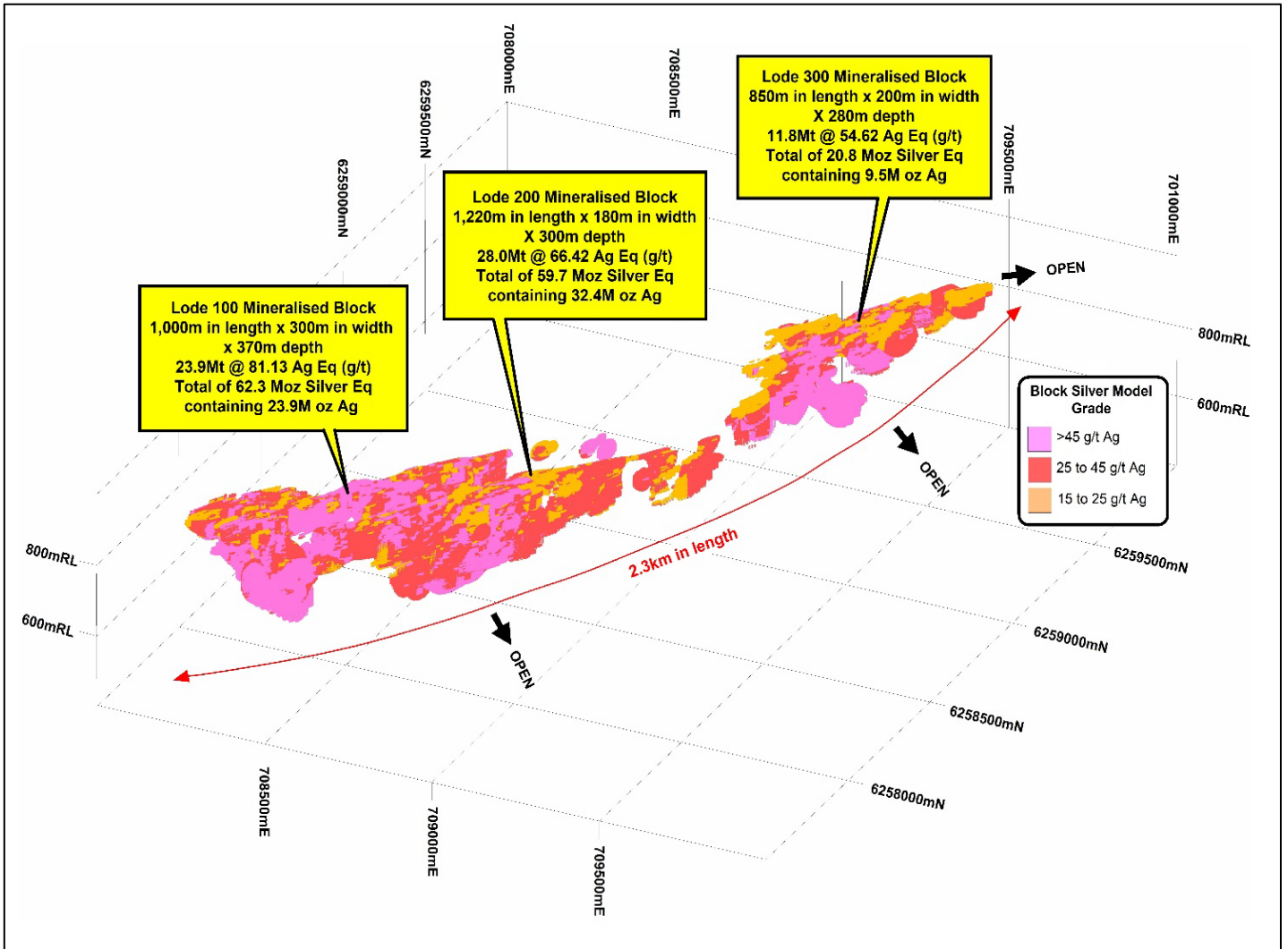
Figure 3 – Oblique 3D Image looking NW of Kempfield outlining the Dimensions & Grade of Mineralised Block Model
