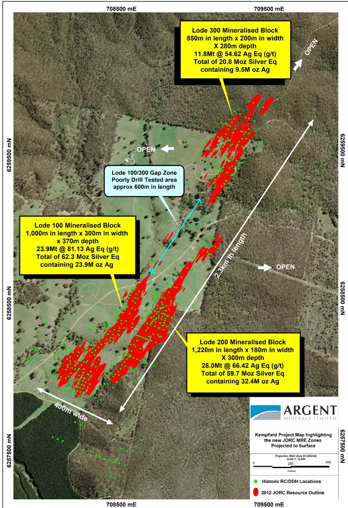
Figure 2 – Kempfield Project Location Map highlighting New 2012 JORC MRE Zones
