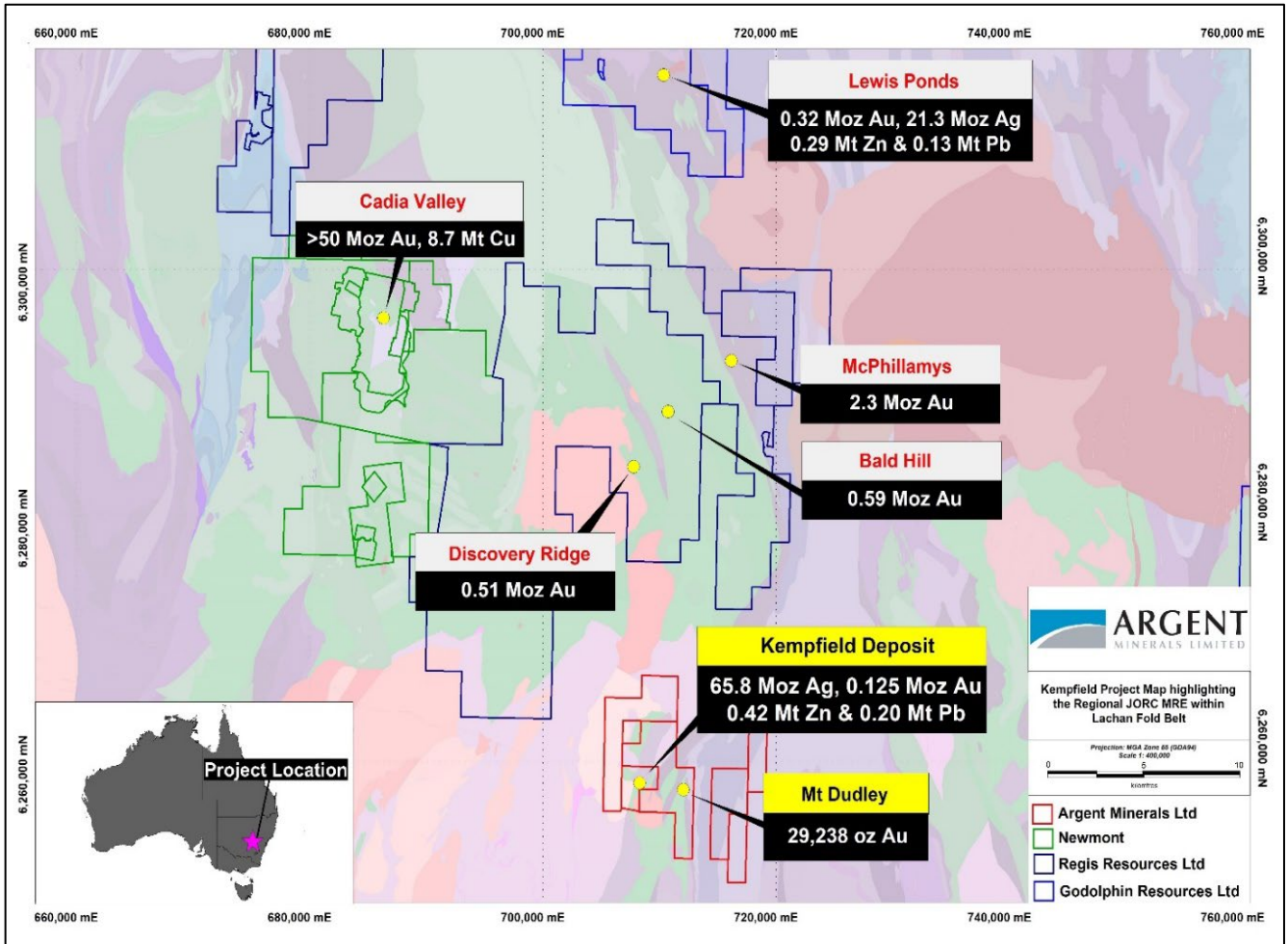
Figure 1 – Regional Kempfield Project Location Map highlighting surrounding nearby Resources
