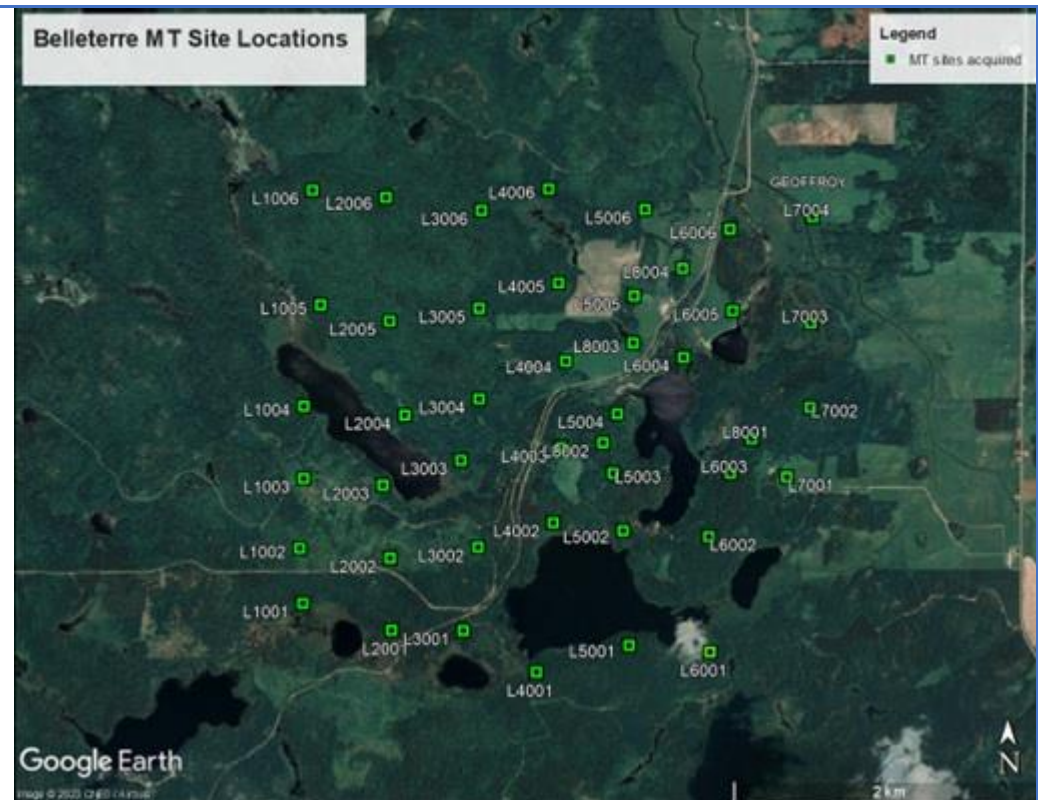
Figure. AMT points on seven lines surveyed by MoomBarriga GeoScience, 44 points.
