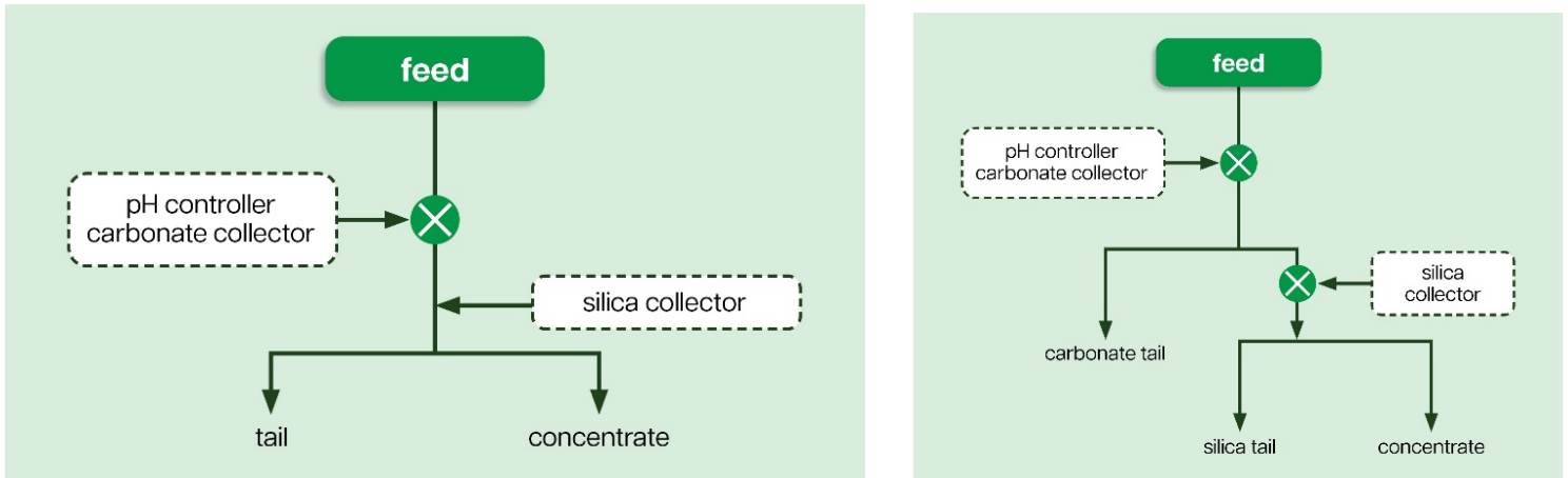
Figures 2a and 2b. Schematic Single Stage Flotation versus Two Stage Flotation
