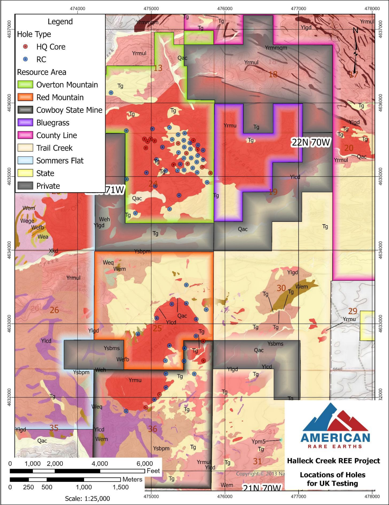
Figure 1 – Locations of Holes used for UK Testing
