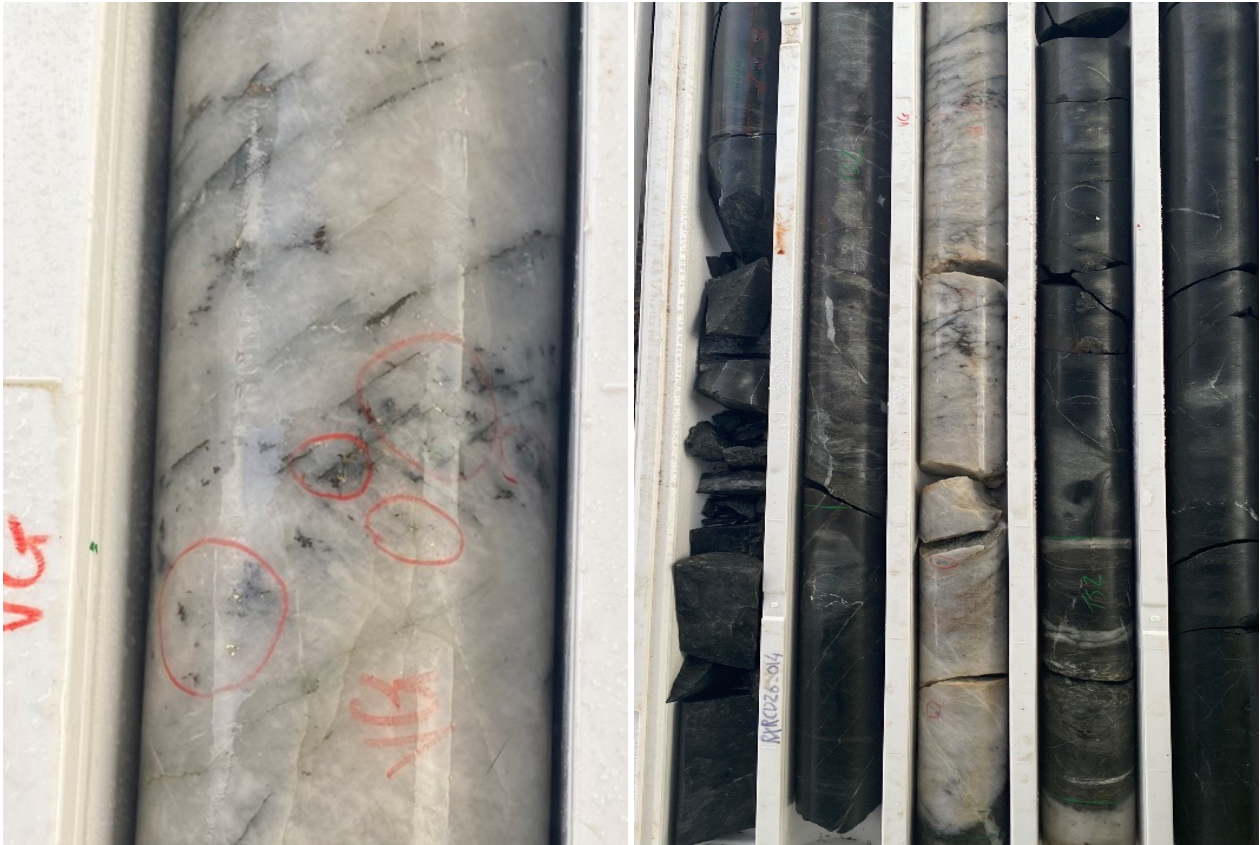
RXRCD014: 2.01 m @ 82.99 g/t Au incl. 1.00 m @ 165.0 g/t Au from 636.05 m. Visible Au from within the laminated quartz vein.
