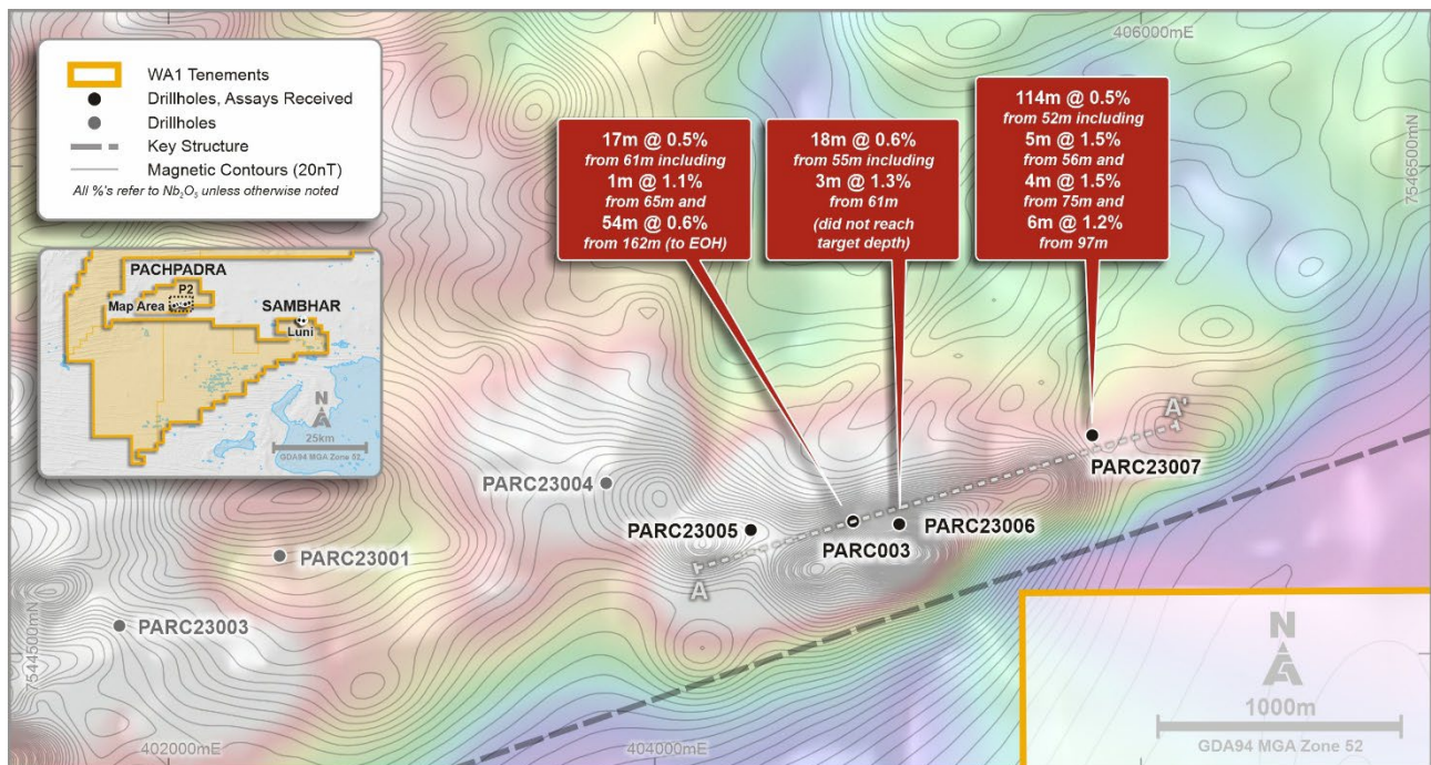
Figure 7: Plan view of the P2 drill collar locations
