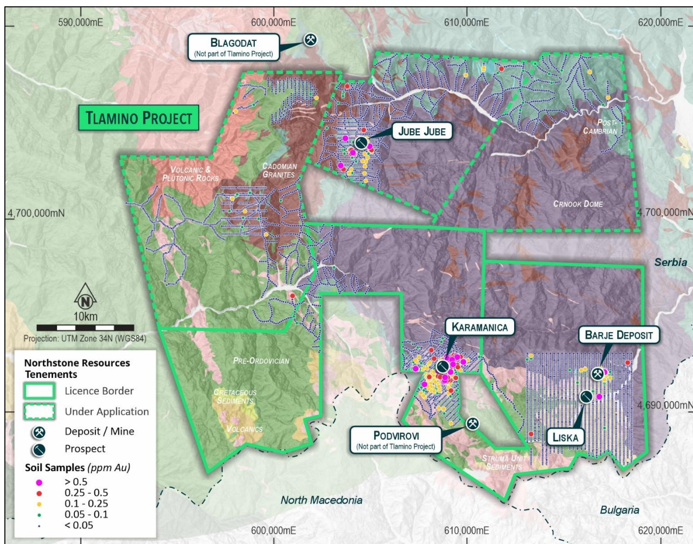
Figure 2 - Overview of Tlaminio Project, Showing Permit Areas, Key Targets and Significant Historic Sampling Results
