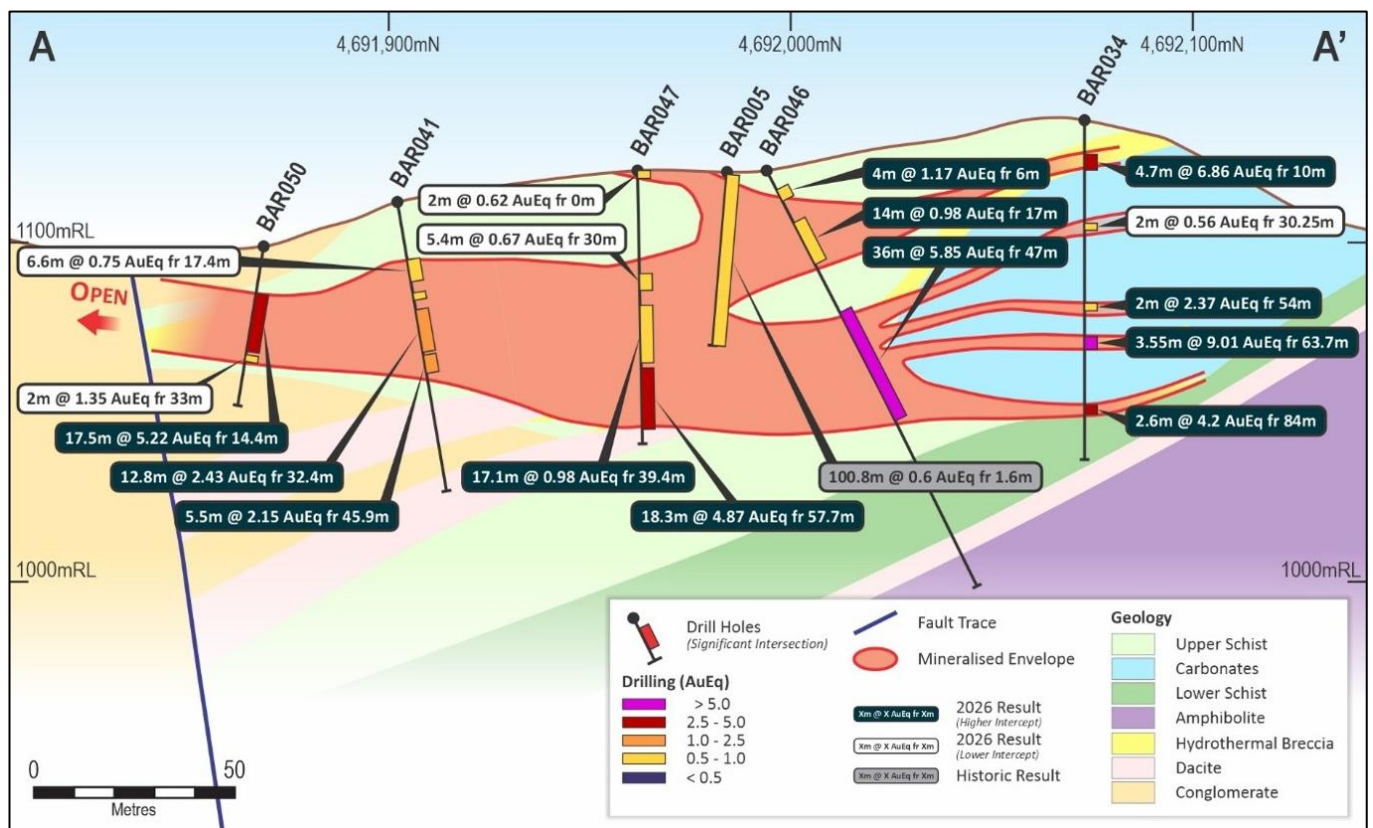
Figure 3 - Barje Cross-Section A-A' Showing 2026 Results for BAR034, BAR041, BAR046, BAR047 and BAR050
