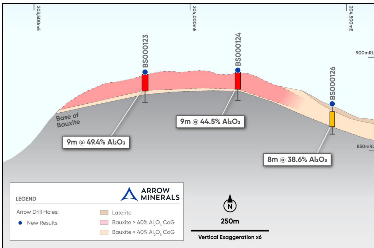
Figure 4. Boussoura North-West Drill Section 1,206,550 North, analytical results reported as significant intercepts with 40% Al 2 O 3 (red) and 37% Al 2 O 3 (orange) cut-off looking North
