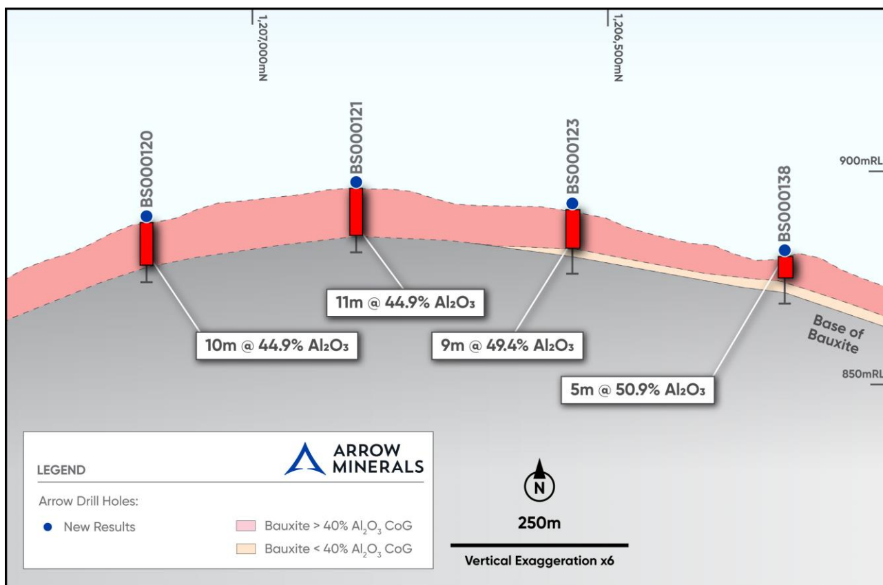
Figure 3. Boussoura North-West, Drill Section 203,850 East, analytical results reported as significant intercepts with a 40% Al 2 O 3 cut-off looking East
