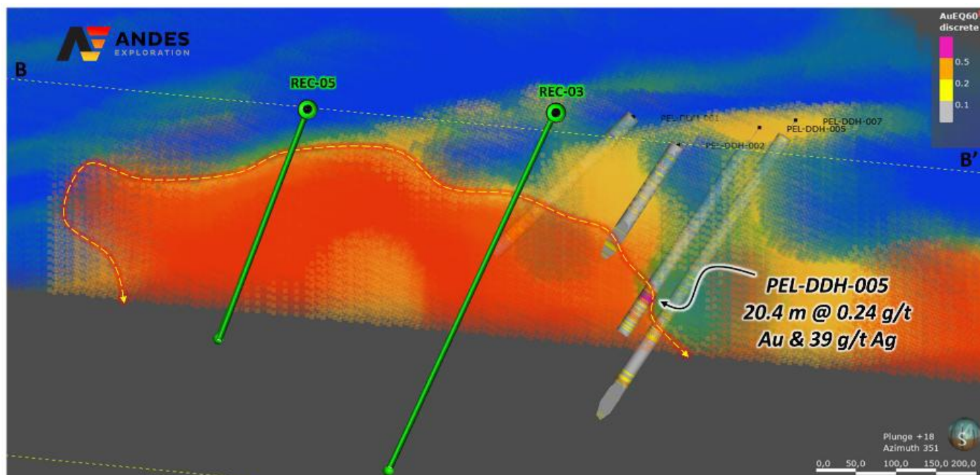
Figure 16 – Longitudinal section through the Marcelina prospect showing historical drilling, the interpreted chargeability anomaly beneath the preserved silica cap and the proposed REC-03 and REC-05 drill holes targeting the concealed sulphide-rich feeder zone.
