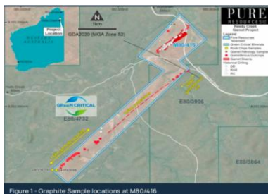
Fig. 1 Graphite sample locations at M80/416, Reedy Creek Garnet Project (GDA2020, MGA Zone 52).
