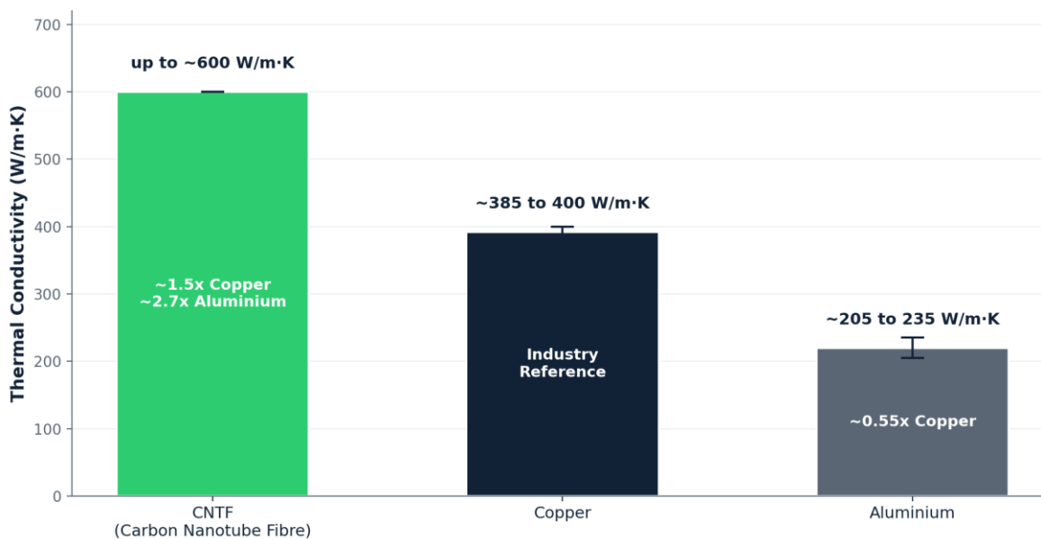
Figure 1: Thermal Conductivity: CNTF vs Copper and Aluminium.
