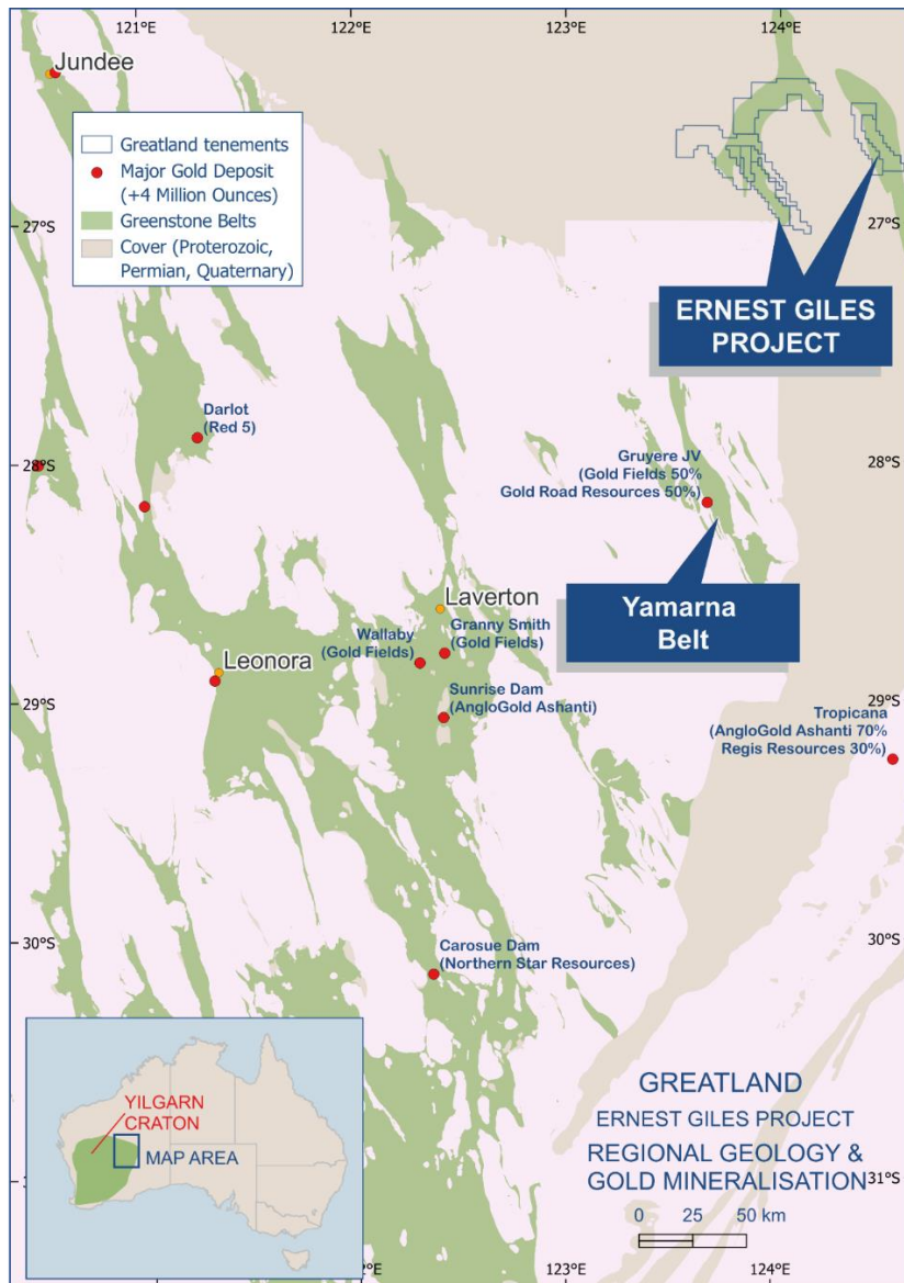
Figure 24: Ernest Giles Project and Yamarna Belt location
