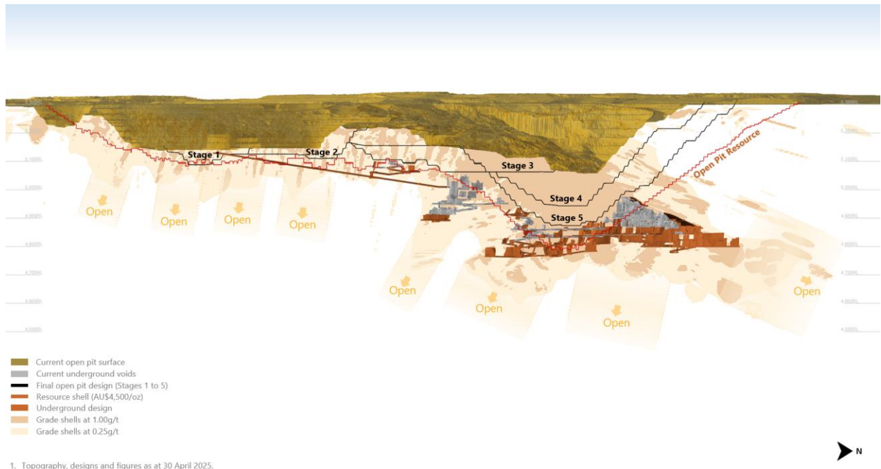
Figure 1: KoTH open pit Ore Reserve by stage with underground LOM design and larger A$4,500/oz Mineral Resource shell
