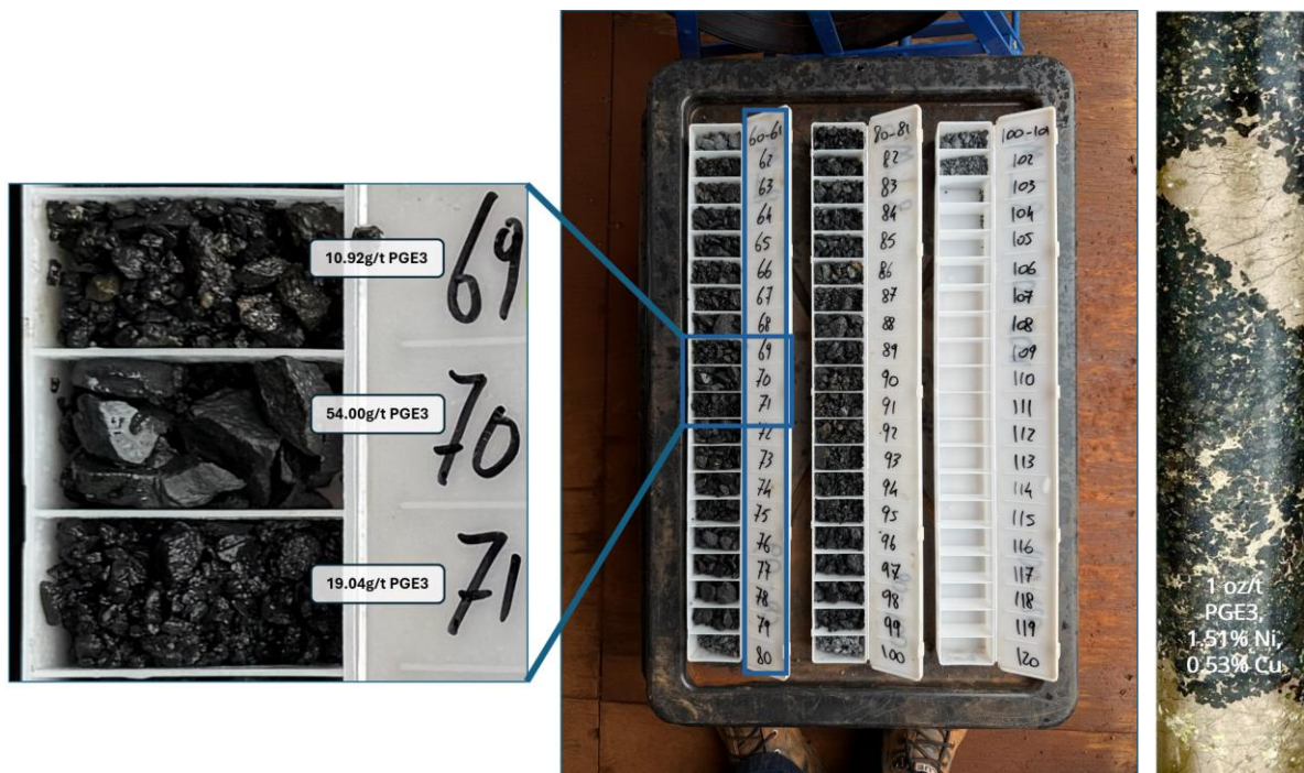
Figure 2. Drill core from hole SWDD006 (226.6 – 226.9 m) which reported 1.00 oz/t PGE3, 1.5% Ni, and 0.53% Cu (right); and RC chip from the ultra-high grade SWT008 discovery hole which reported up to 54g/t PGE3 (left).
