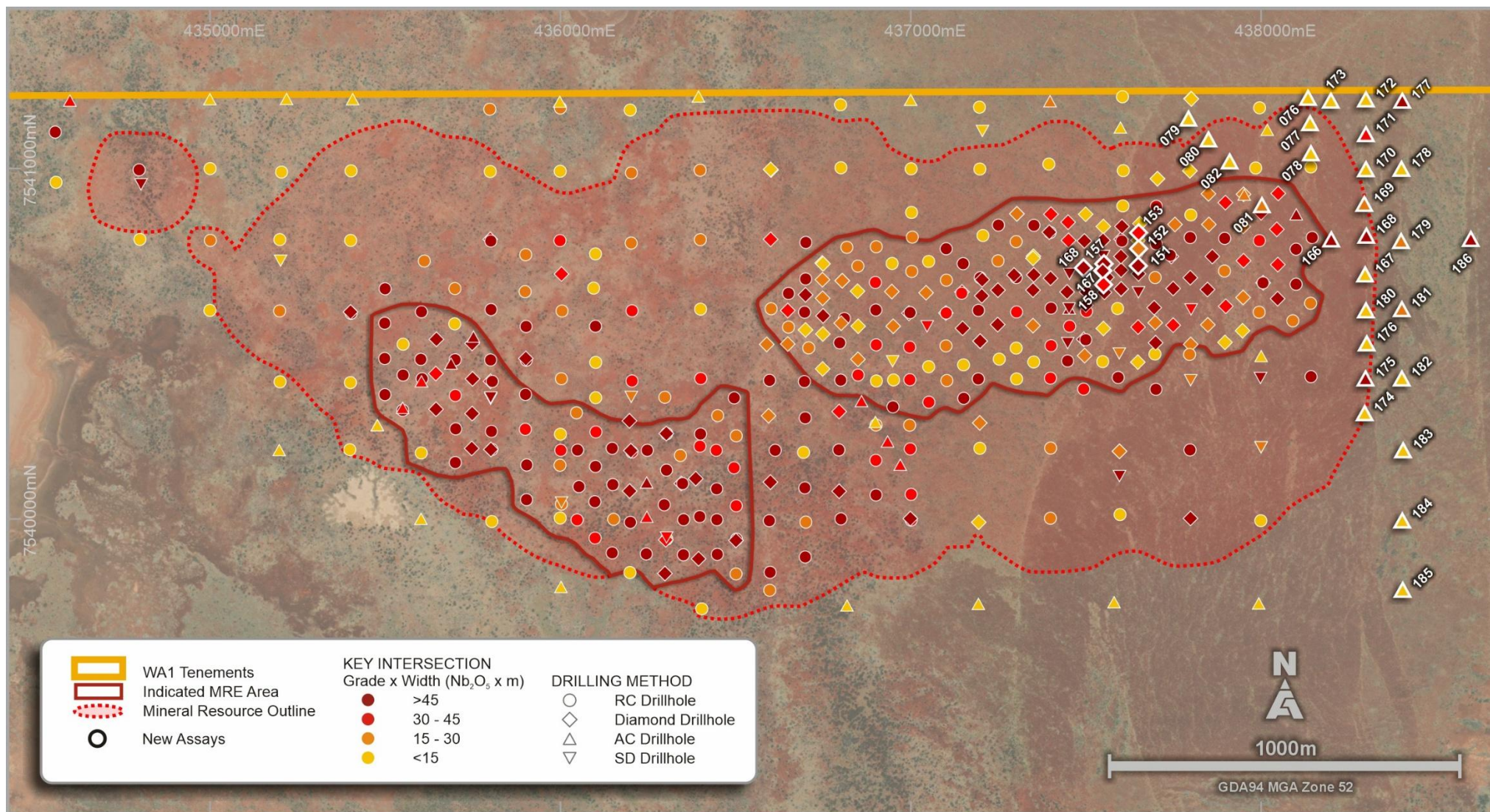
Figure 5: Luni niobium deposit plan view of completed drilling with grade by width intersections reported to date
