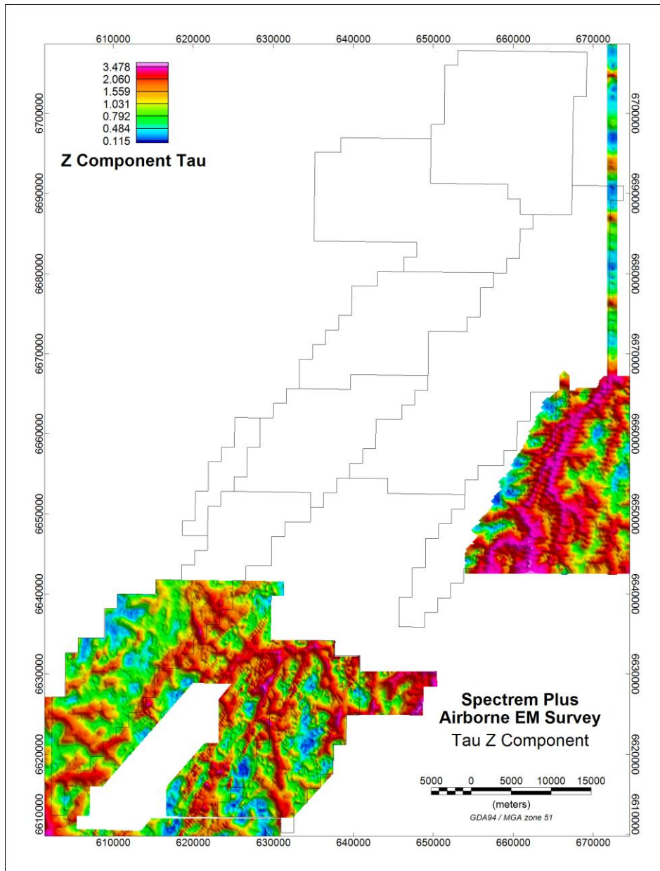
Figure 14: Spectrem Plus EM survey over Plumridge Nickel JV tenements
