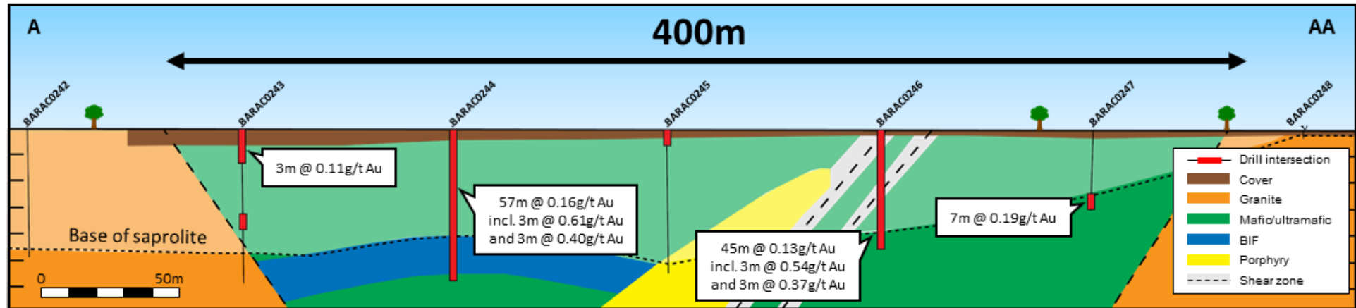
Figure 7: T8 Prospect – cross section through A-AA (Figure 6)
