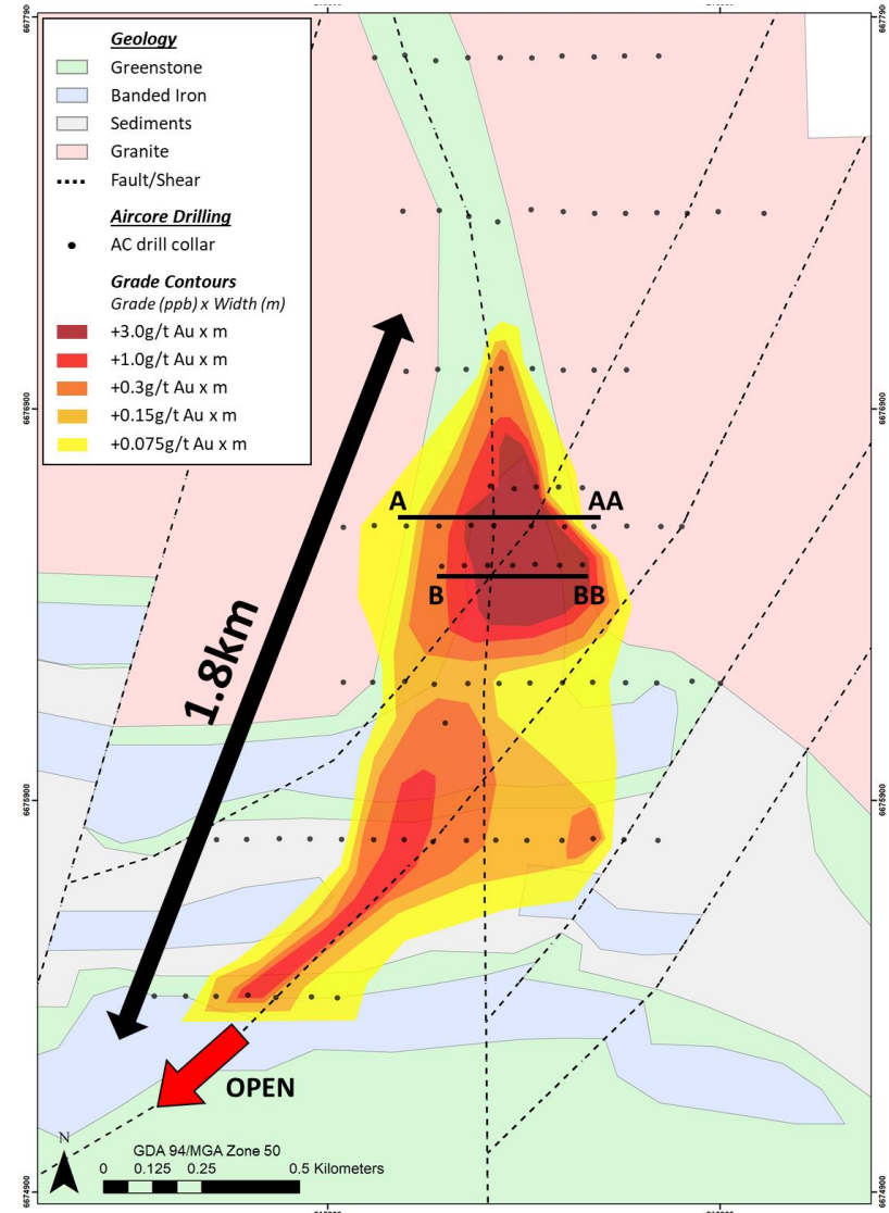
Figure 6: T8 Prospect – aircore drilling gold anomaly (ppb Au x metre contours)
