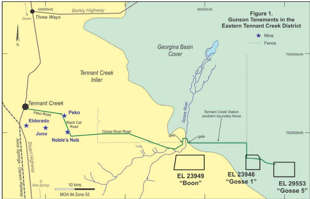
Figure 1 Gunson Tenements in the Eastern Tennant Creek District
