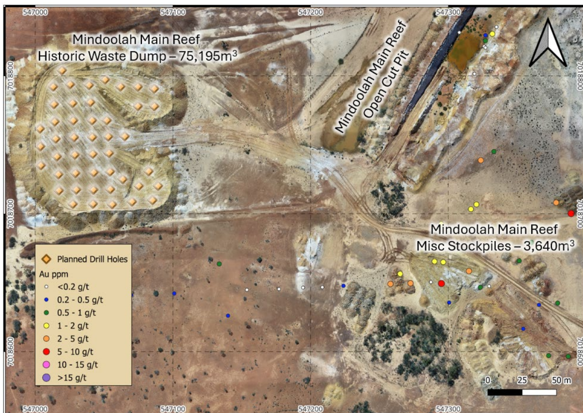
Figure 2. Mindoolah Main Reef Waste Dump Drill Program locations with Historic Rock Chip Grab Samples as coloured dots in surrounding areas (Appendix 1: Table 2).
