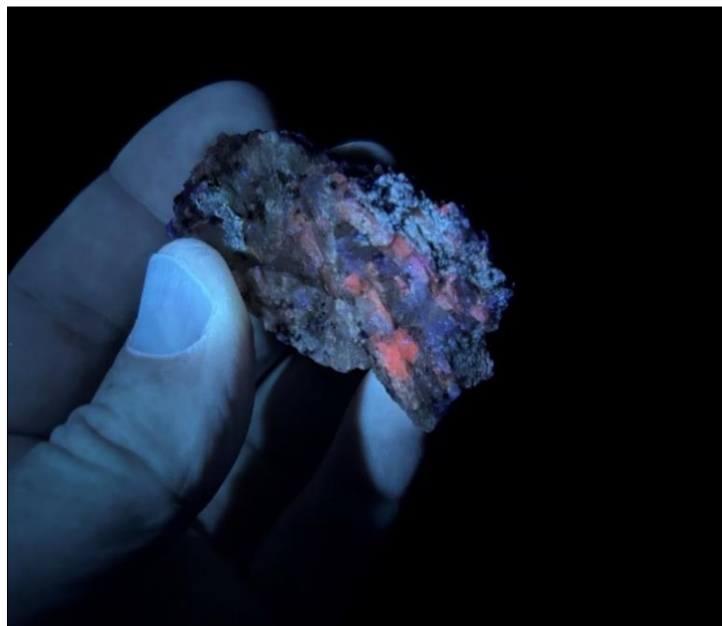
Figure 5: Weathered LCT pegmatite identified from the northern Widgiemooltha project area (UV light 365nm)
