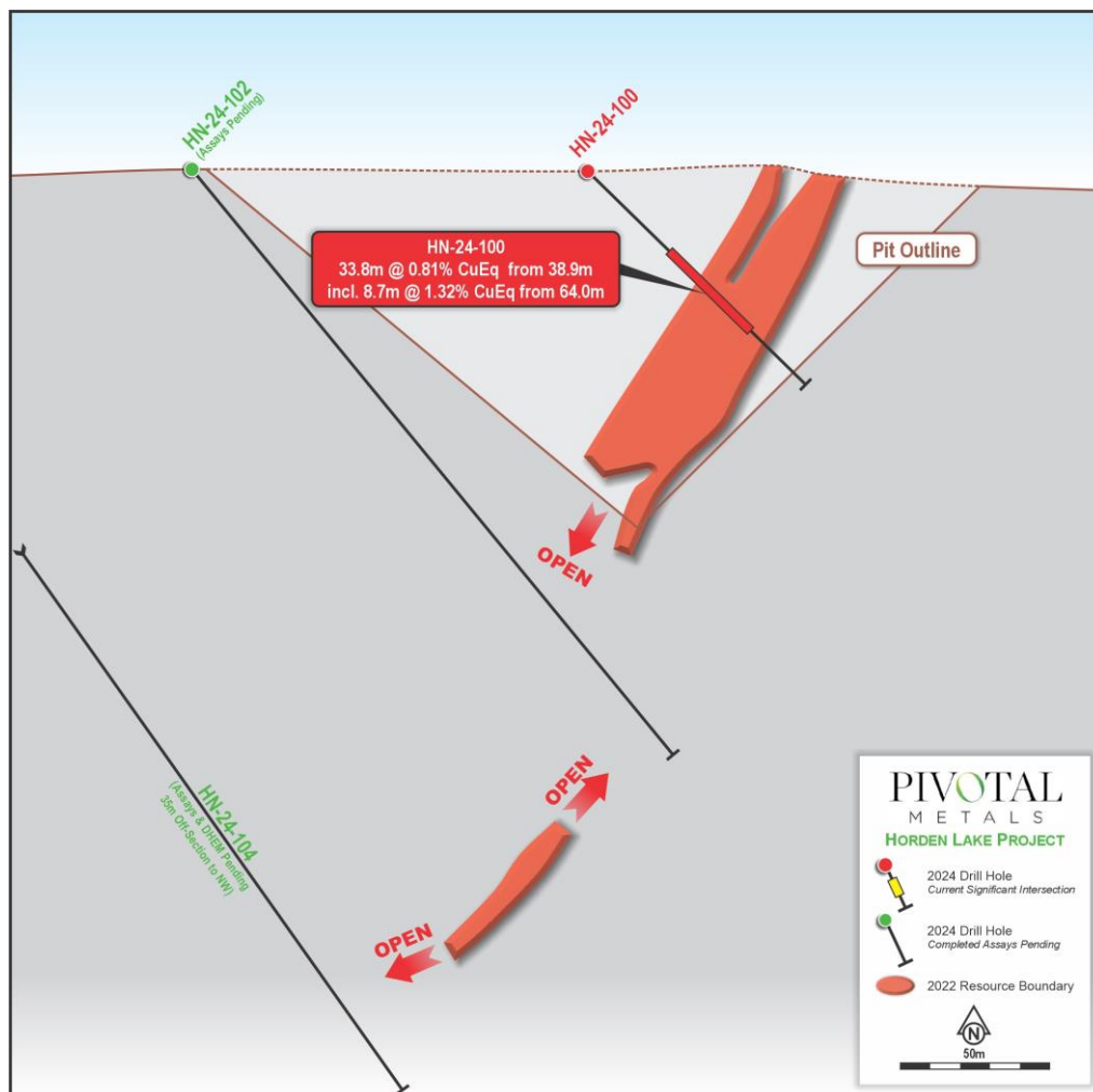
Figure 5: Cross section through HN-24-100 ( \pm 10\text{m} ), Hornden Lake deposit
