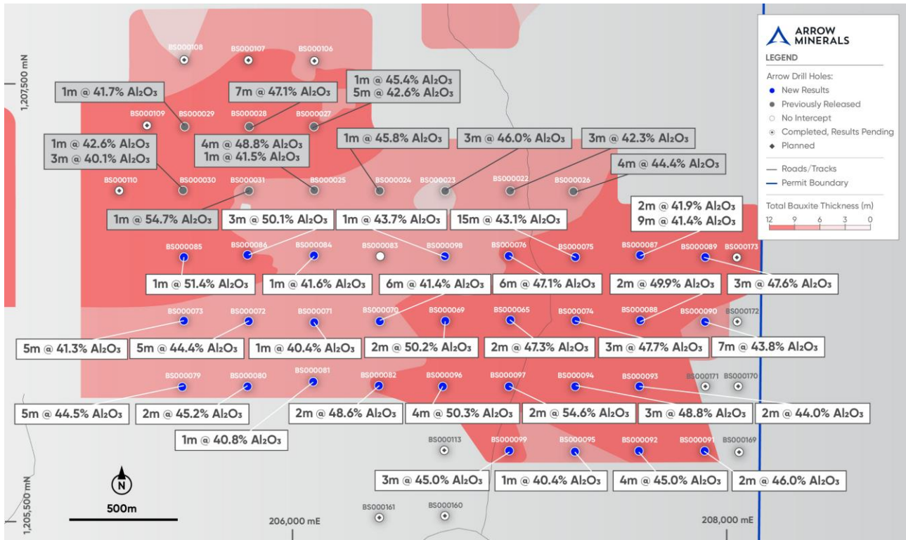
Figure 3. Boussoura Central analytical results reported as significant intercepts with a 40% Al 2 O 3 cut-off, overlain on total bauxite thickness from logged geology, and SRTM topography
