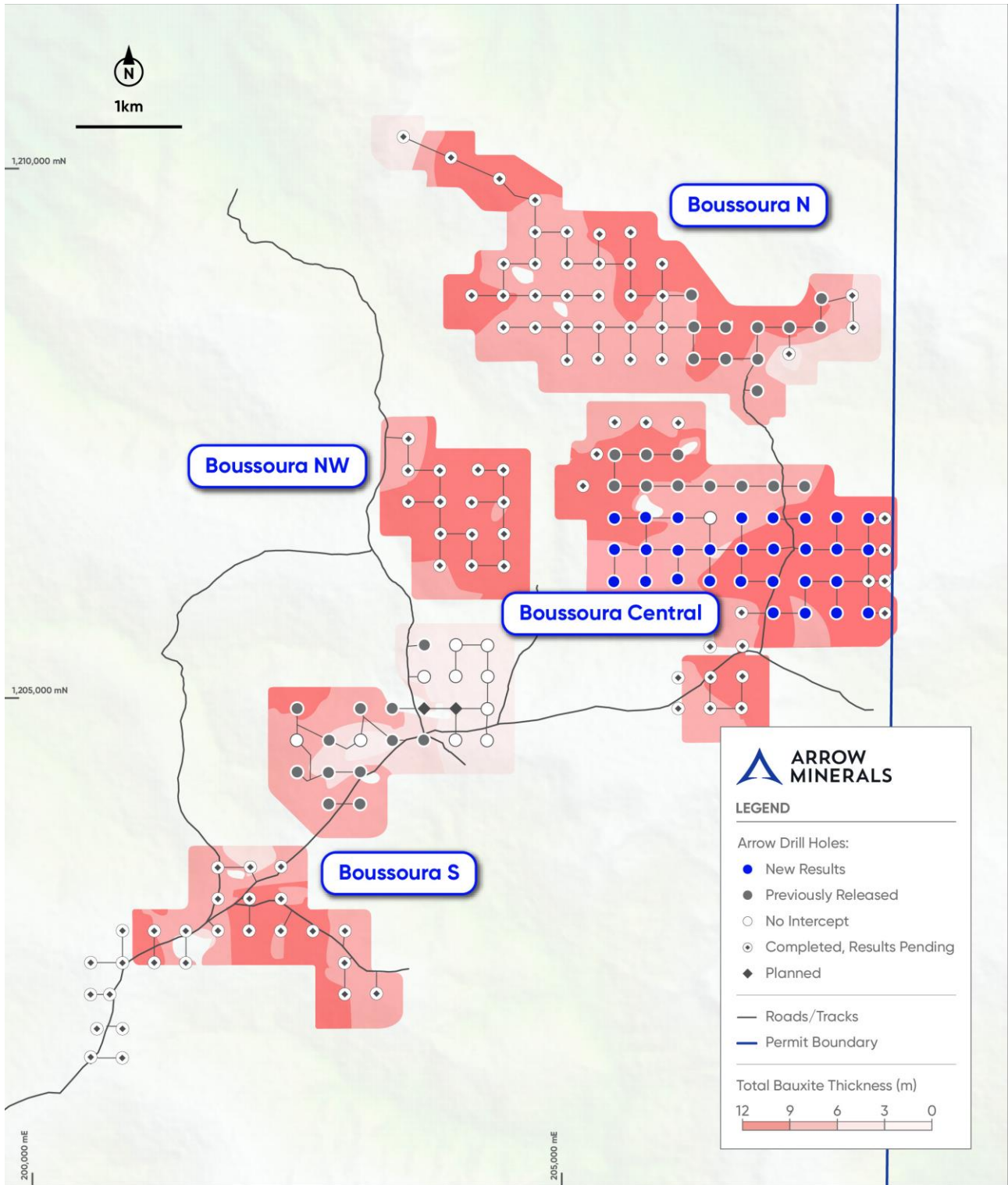
Figure 2. Drill Status Plan showing total bauxite thickness from logged geology, and SRTM topography.
