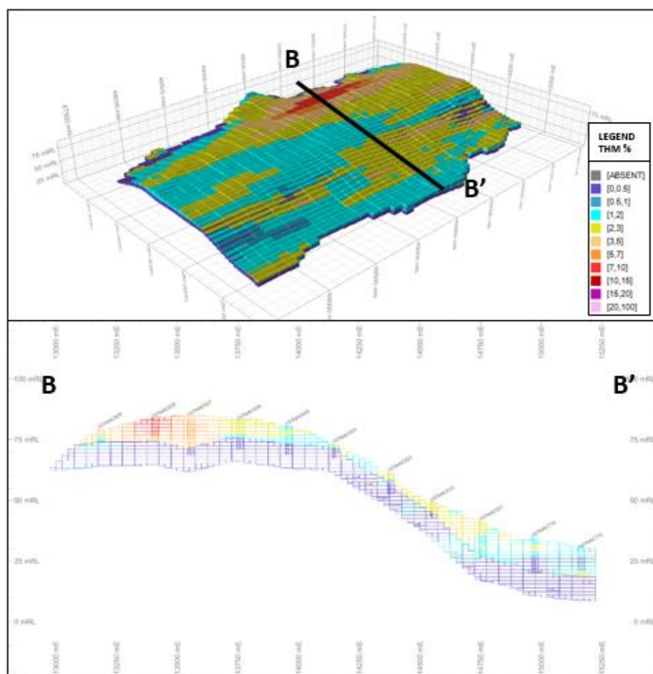
Figure 9 Tajiri North Resource Block Model and Cross-Section (looking north x10 VE)
