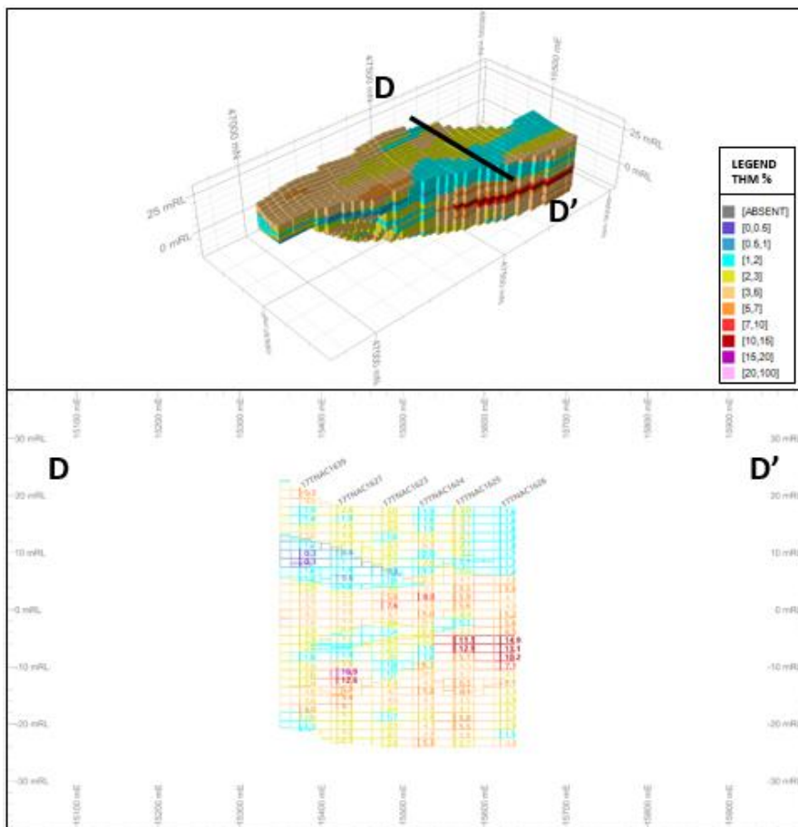
Figure 17 T4C Channel Resource Block Model and Cross-Section (looking north x7 VE)
