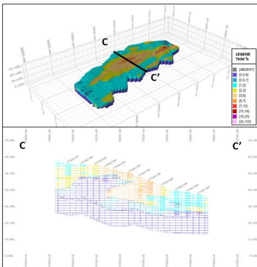
Figure 11 T2 Resource Block Model and Cross-Section (looking north x7 VE)
