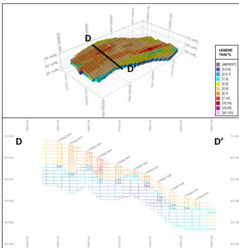
Figure 13 T3 Resource Block Model and Cross-Section (looking north x7 VE)
