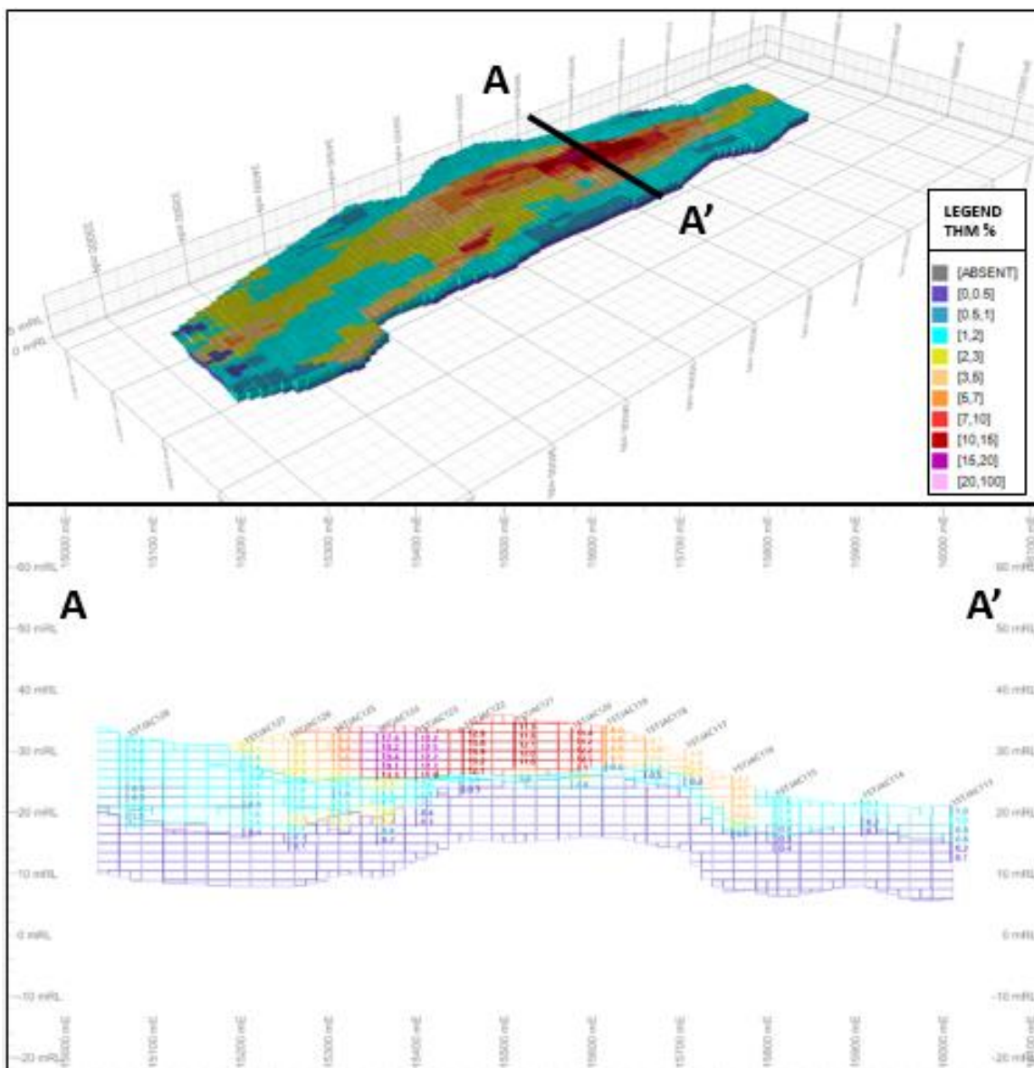
Figure 7 Tajiri Resource Block Model and Cross Section (looking north x7 vertical exaggeration)
