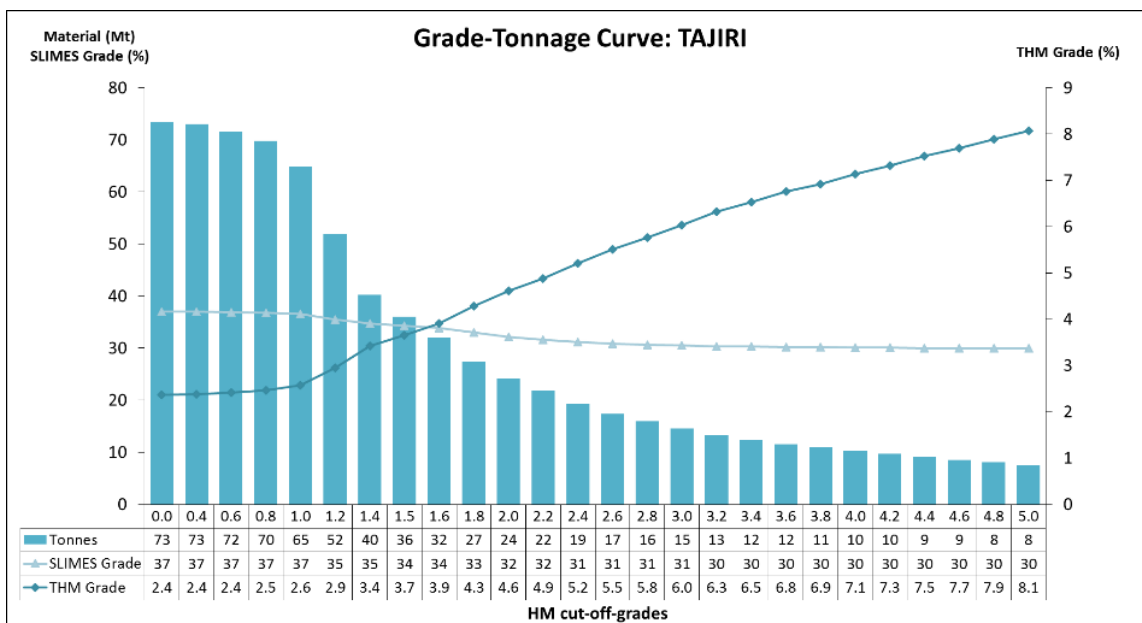
Figure 6 Tajiri Resource Grade-Tonnage Curve
